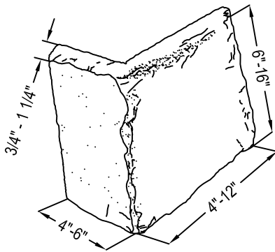
CORNER DETAIL
