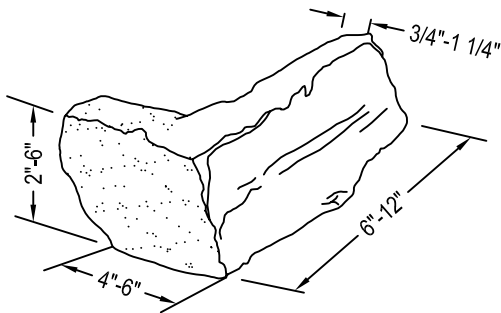
CORNER DETAIL
