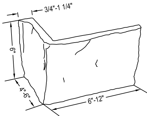
CORNER DETAIL
