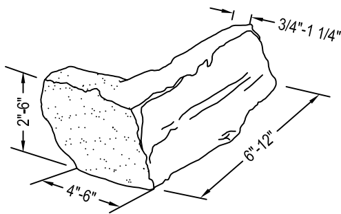
CORNER DETAIL
