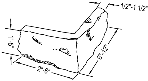
CORNER DETAIL
