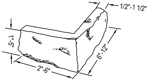
CORNER DETAIL
