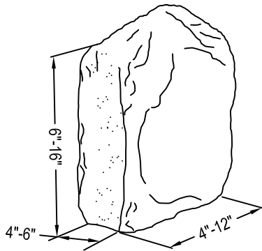
CORNER DETAIL
