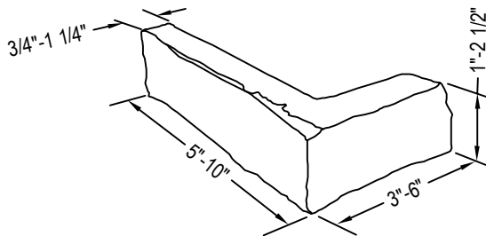
CORNER DETAIL
