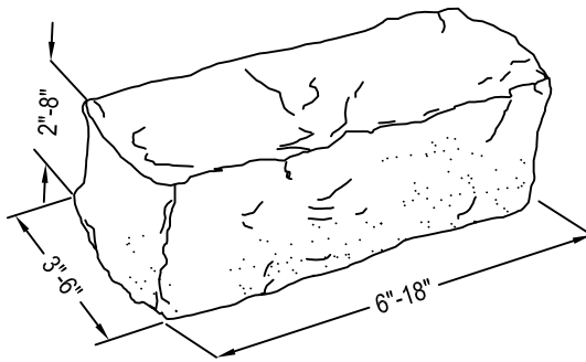
FLAT DETAIL
